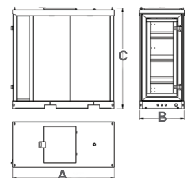
Tank dimensions
